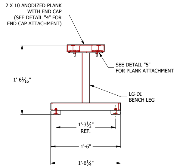
RUBBER FOOT PAD OPTION SEE DETAIL "1"
