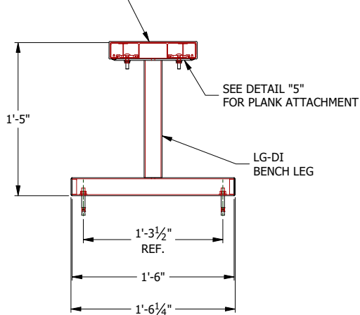
CONCRETE ANCHOR OPTION SEE DETAIL "3"
